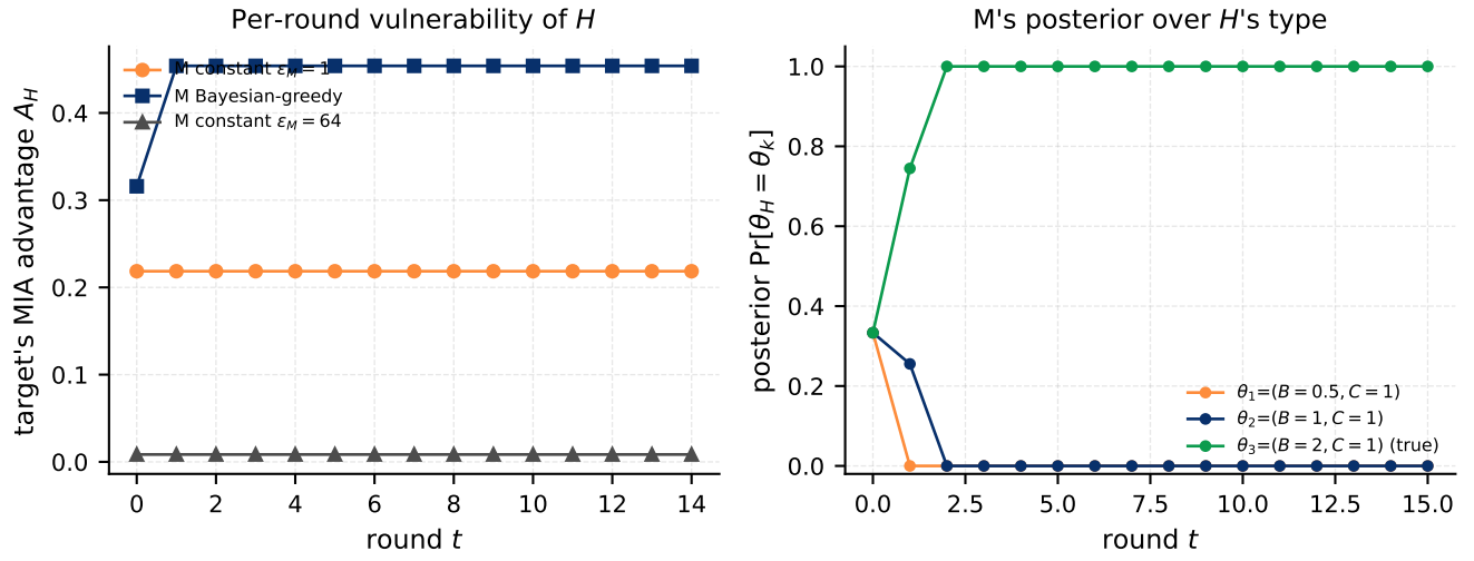
Fig. 8: BR-PEG demo . Left: per-round realised MIA advantage A_H of the honest player under three M policies. Right: M's posterior over H 's type under the Bayesian-greedy policy; the posterior collapses to the true type within two rounds.
