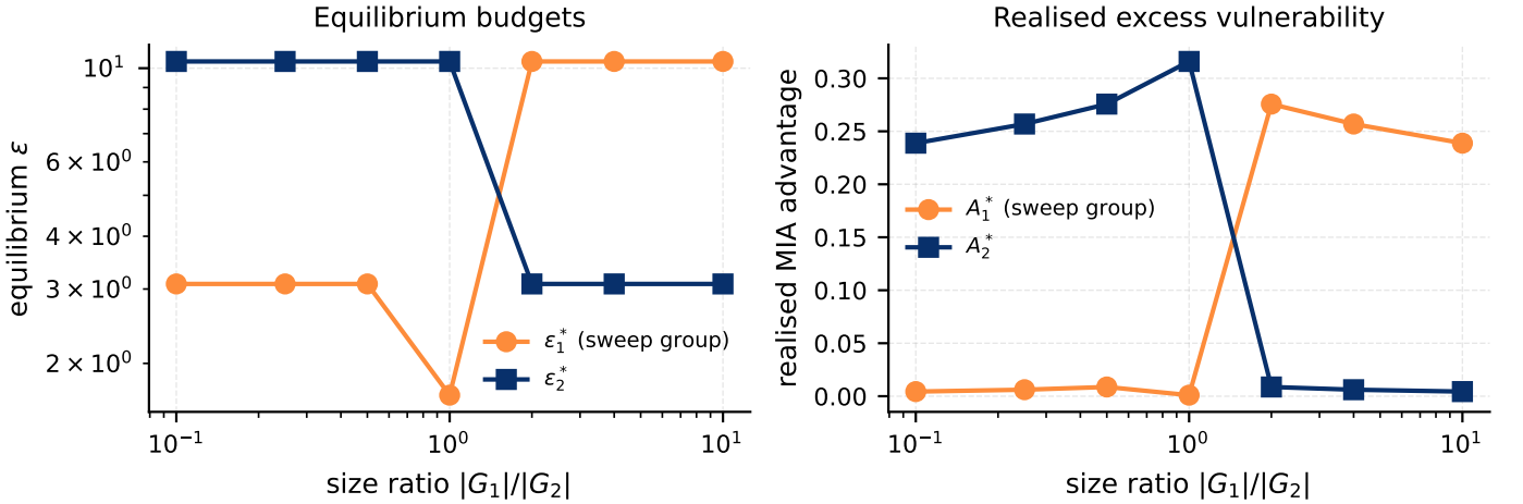
Fig. 2: C2. Equilibrium budget (left) and realised MIA advantage (right) as a function of dataset size ratio |G_1|/|G_2| . The minority group's \varepsilon^* is always lower than the majority's, and its realised A^* correspondingly smaller. The flip at r=1 is the boundary at which the minority/majority labels exchange.
