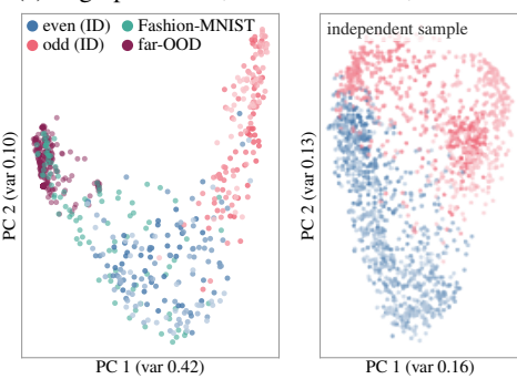
(e) fingerprint PCA, 75-d FFN act., 64-d
