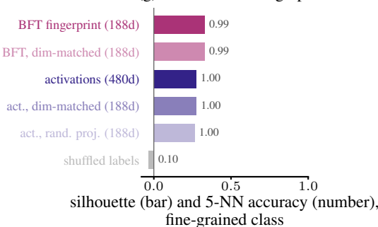
(g) vs. baselines: fingerprint or activations
