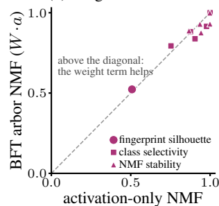
(h) weights vs. activations only
