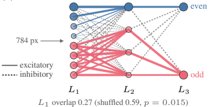
(a) the two class circuits
