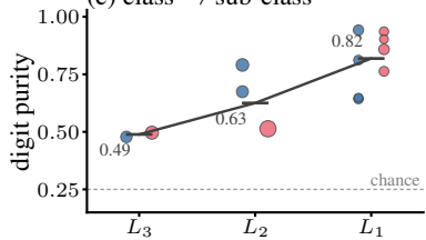
(c) class → sub-class
