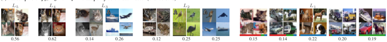
(c) traced spine of f_9 , L_5 \rightarrow L_1 — class purity below each factor (chance 0.10)
