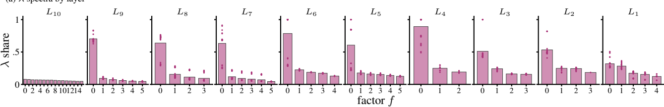
(a) \lambda spectra by layer
