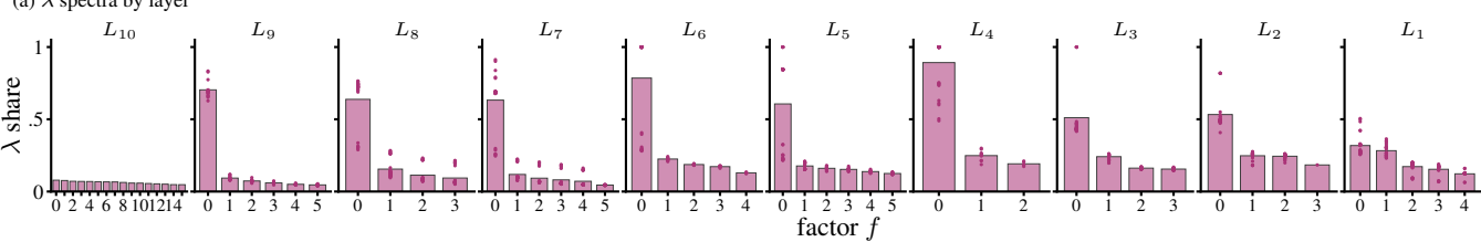
(a) \lambda spectra by layer
