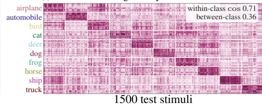
(i) both · fingerprint vs. activations
