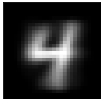
inh factor 1 \lambda=0.19 weighted avg
