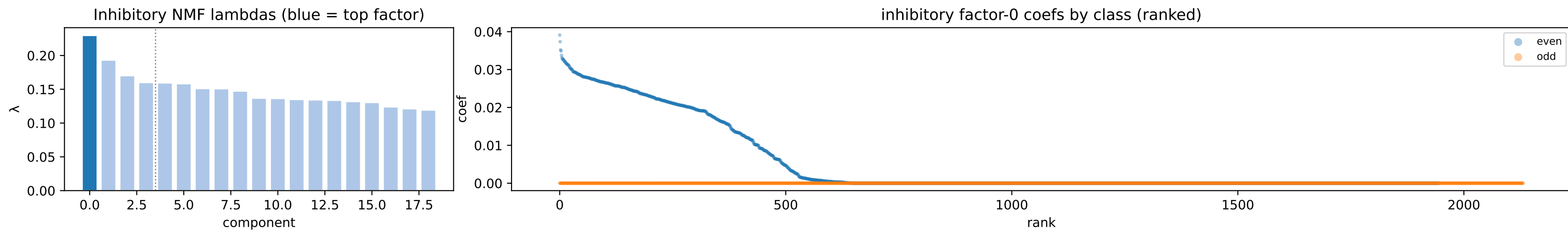
inh factor 0 \lambda=0.23 weighted avg
