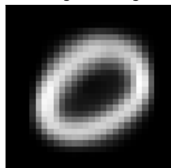
inh factor 2 \lambda=0.17 weighted avg
