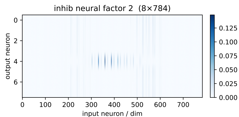
inh factor 2 \lambda=0.17 weighted avg
