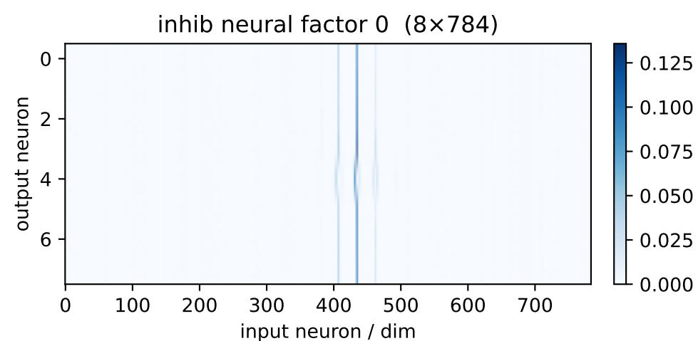
inh factor 0 \lambda=0.23 weighted avg
