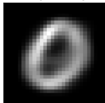
inh factor 3 \lambda=0.16 weighted avg
