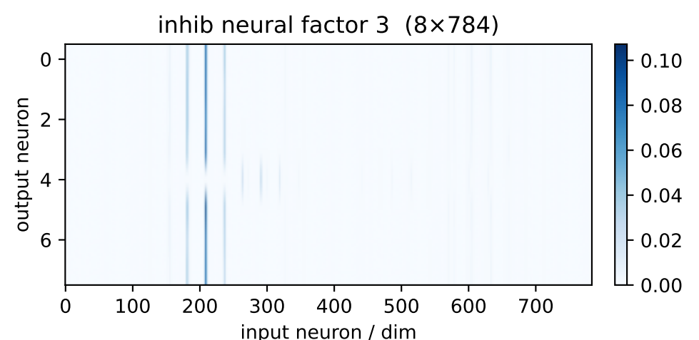
inh factor 3 \lambda=0.16 weighted avg
