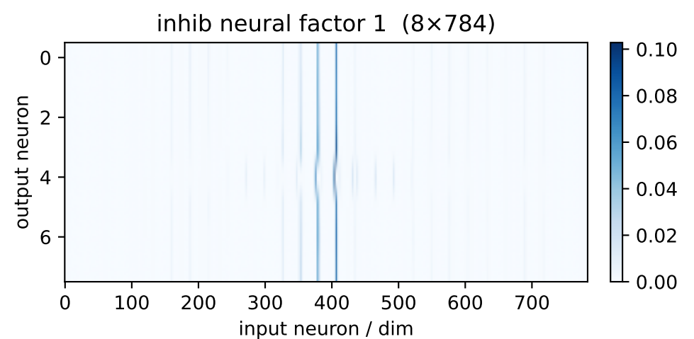
inh factor 1 \lambda=0.19 weighted avg
