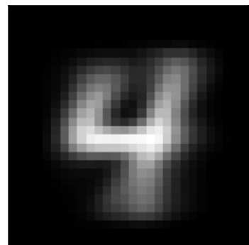
inh factor 0 \lambda=0.23 weighted avg
