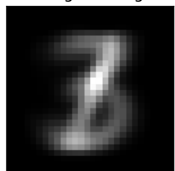
inh factor 3 \lambda=0.27 weighted avg
