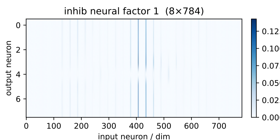
inh factor 1 \lambda=0.31 weighted avg
