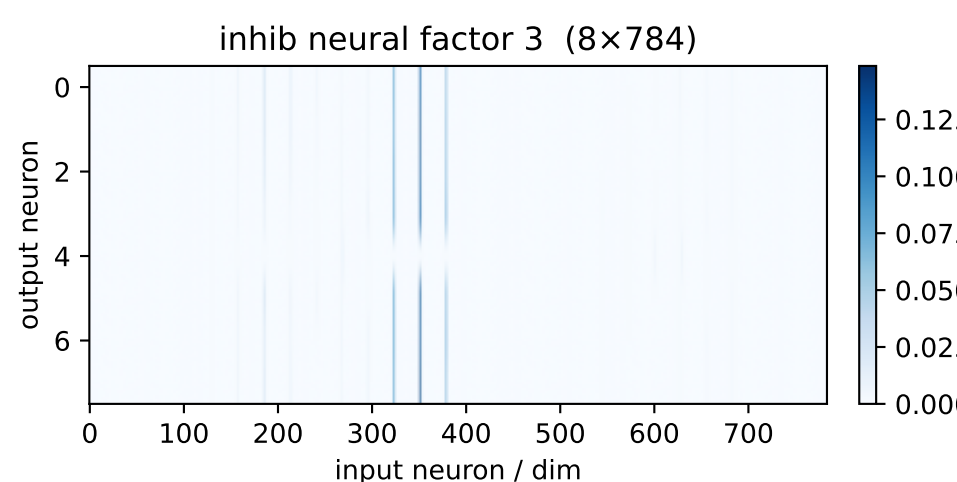
inh factor 3 \lambda=0.27 weighted avg
