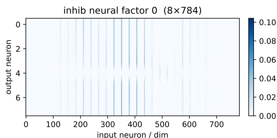
inh factor 0 \lambda=0.37 weighted avg
