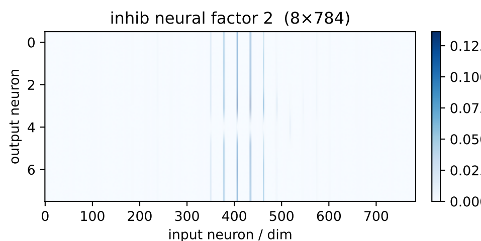
inh factor 2 \lambda=0.28 weighted avg
