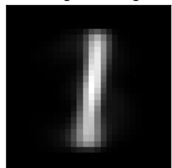
inh factor 0 \lambda=0.37 weighted avg
