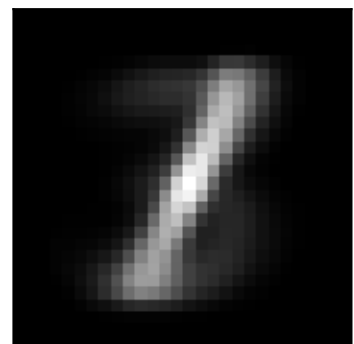
inh factor 1 \lambda=0.31 weighted avg
