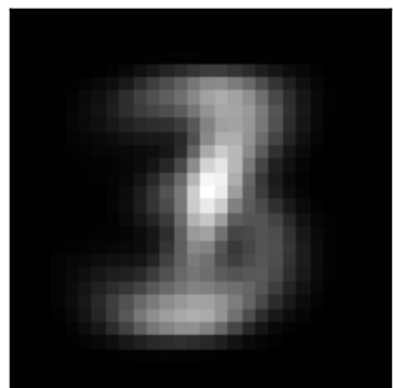
inh factor 0 \lambda=16.06 weighted avg
