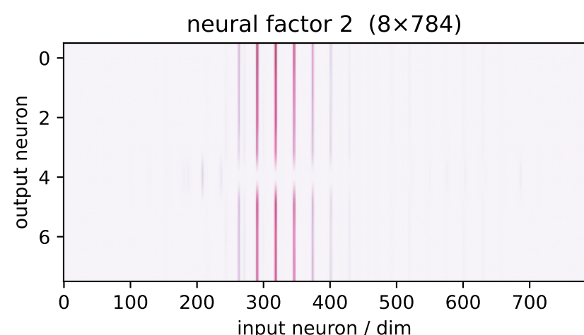
factor 2 \lambda=4.68 weighted avg
