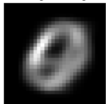
factor 2 \lambda=4.68 weighted avg
