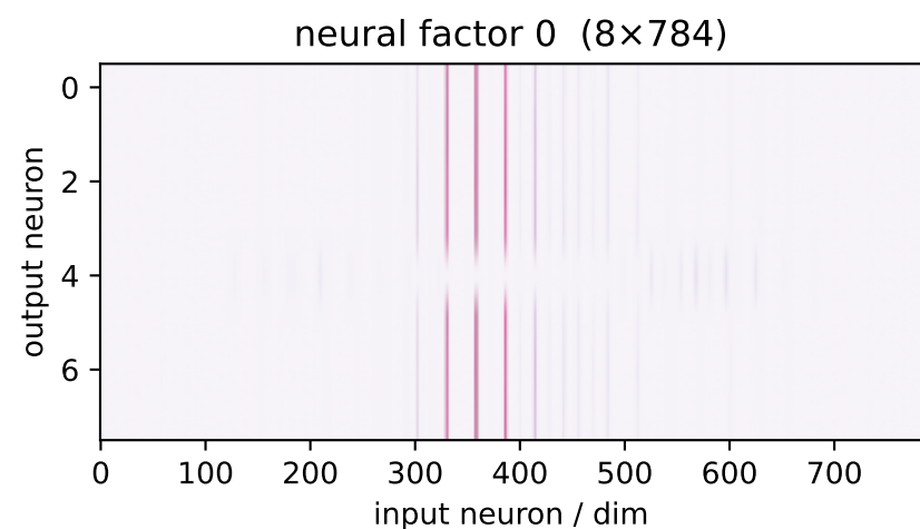
factor 0 \lambda=4.96 weighted avg
