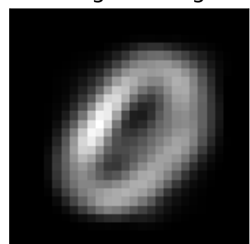
factor 3 \lambda=4.48 weighted avg
