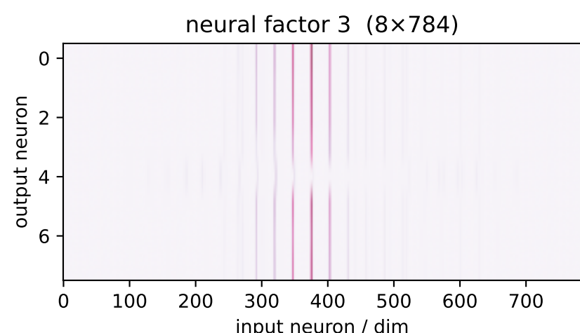
factor 3 \lambda=4.48 weighted avg
