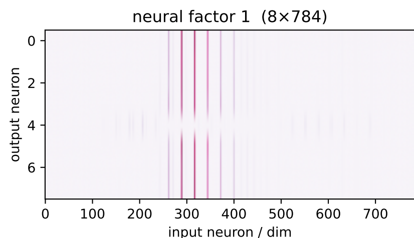
factor 1 \lambda=4.71 weighted avg
