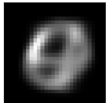
factor 1 \lambda=4.71 weighted avg
