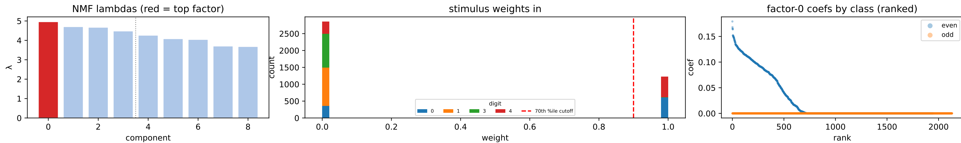
factor 0 \lambda=4.96 weighted avg
