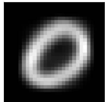
factor 0 \lambda=4.96 weighted avg
