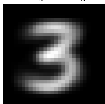
factor 2 \lambda=2.65 weighted avg
