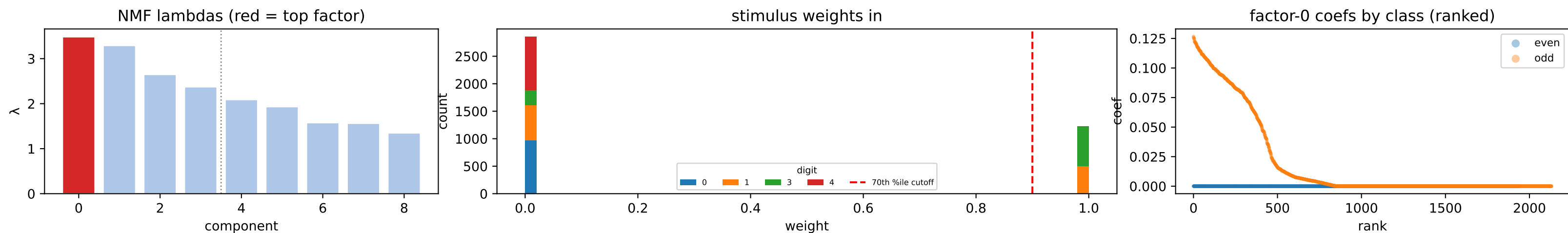
factor 0 \lambda=3.49 weighted avg
