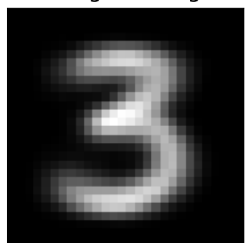
factor 1 \lambda=3.29 weighted avg
