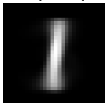
factor 0 \lambda=3.49 weighted avg
