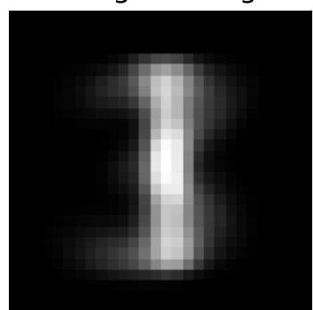
factor 3 \lambda=2.37 weighted avg
