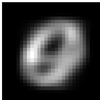
factor 0 \lambda=56.76 weighted avg
