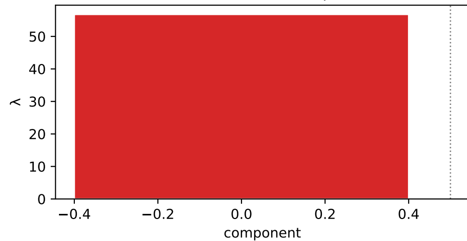
NMF lambdas (red = top factor)
