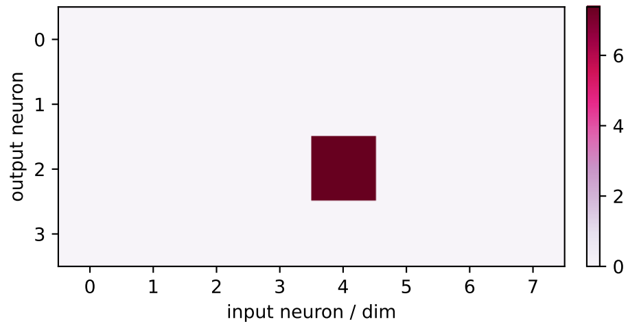
neural factor 0 (4×8)
