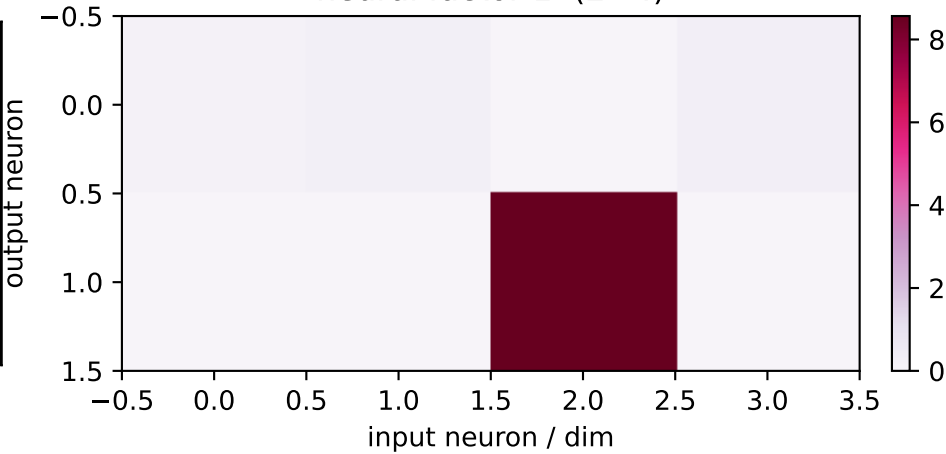
neural factor 1 (2×4)
