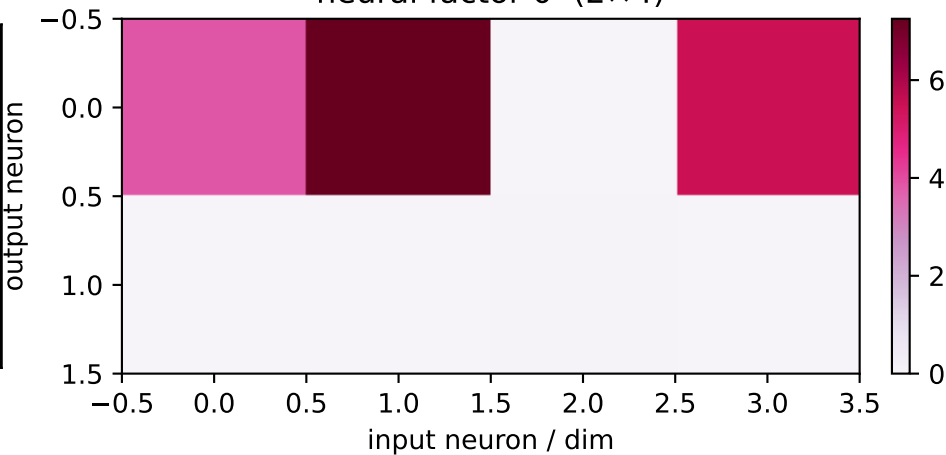
neural factor 0 (2×4)
