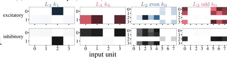
(b) connection maps (out \times in)
