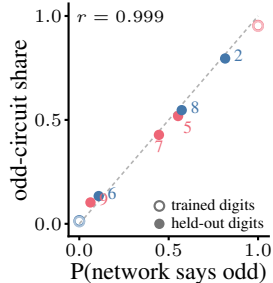
(c) held-out digits
