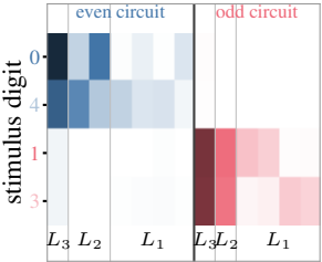
(a) mean fingerprint
