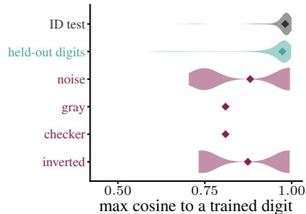
(e) distance to the trained digits
