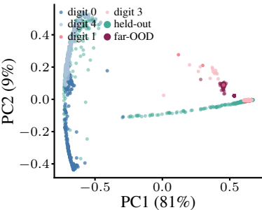
(c) fingerprint PCA
