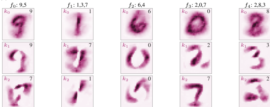
(c) L_1 sub-circuits
