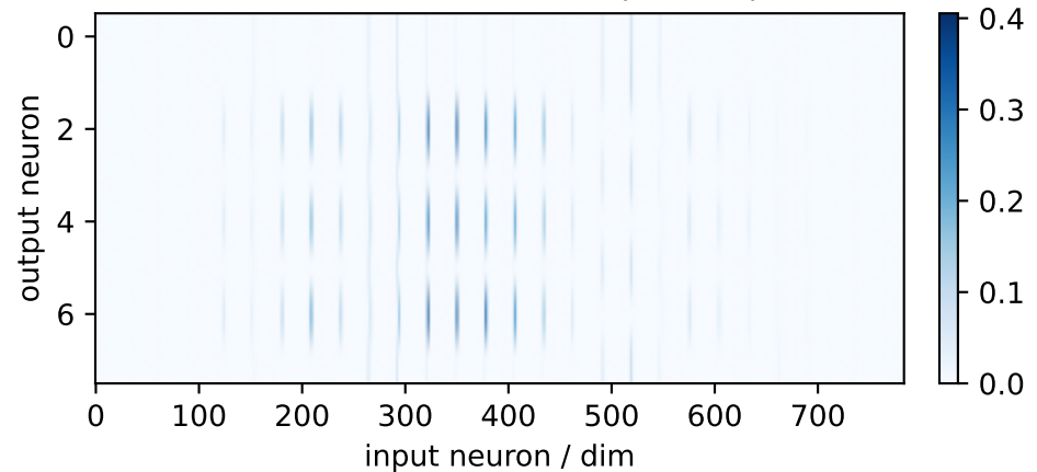
inhib neural factor 2 (8×784)
