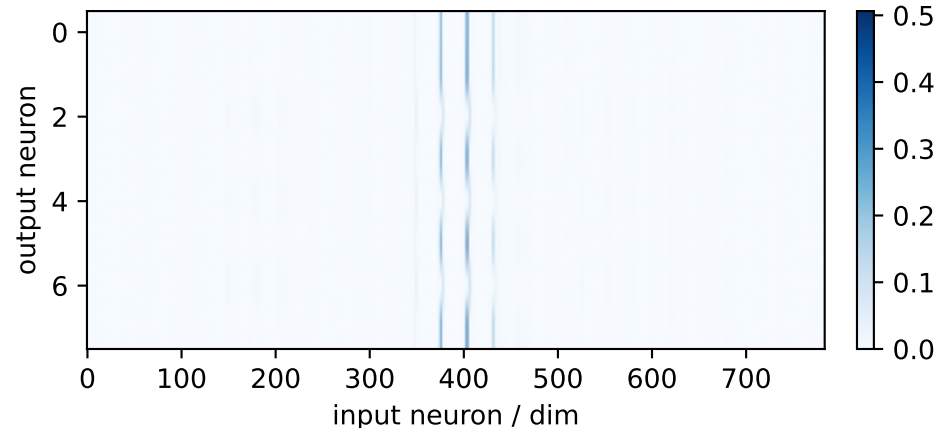
inhib neural factor 3 (8×784)
