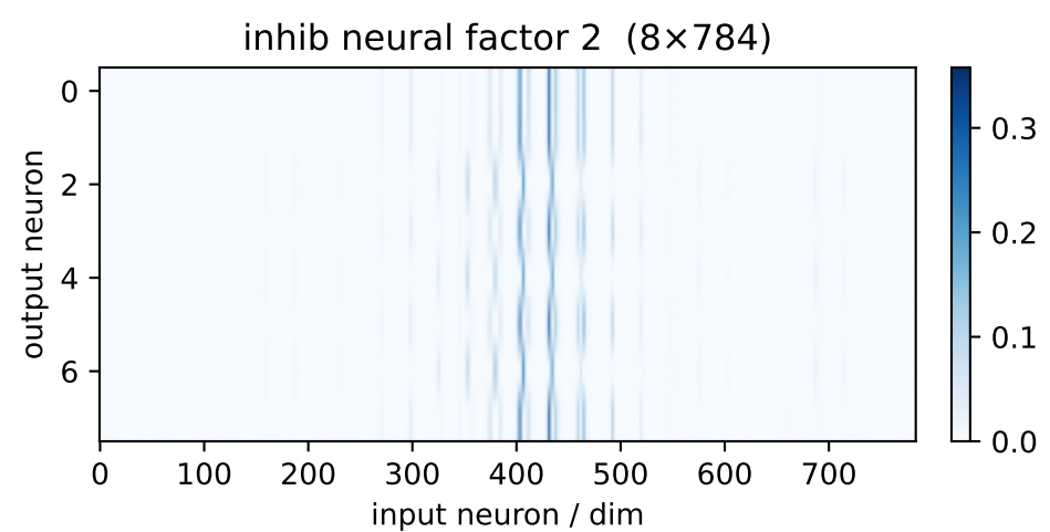
inh factor 2 \lambda=3.55 weighted avg
