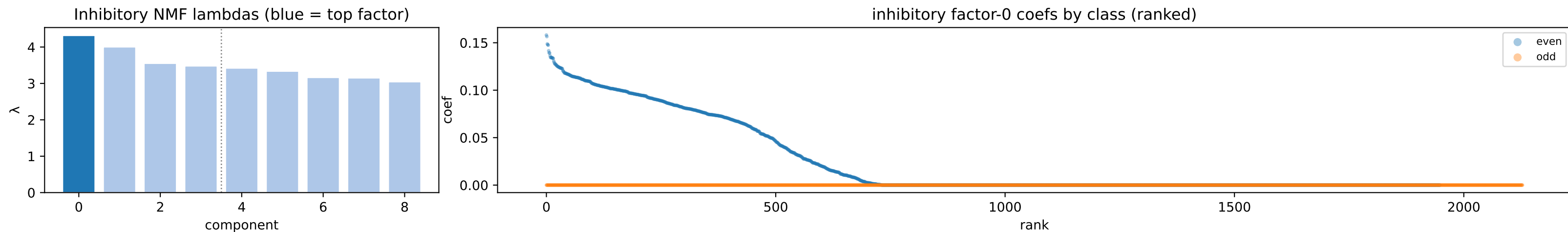
inh factor 0 \lambda=4.32 weighted avg
