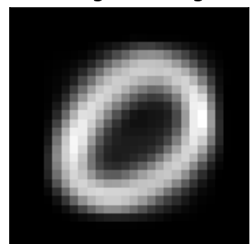
inh factor 0 \lambda=4.32 weighted avg
