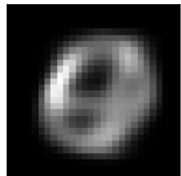
inh factor 1 \lambda=4.00 weighted avg
