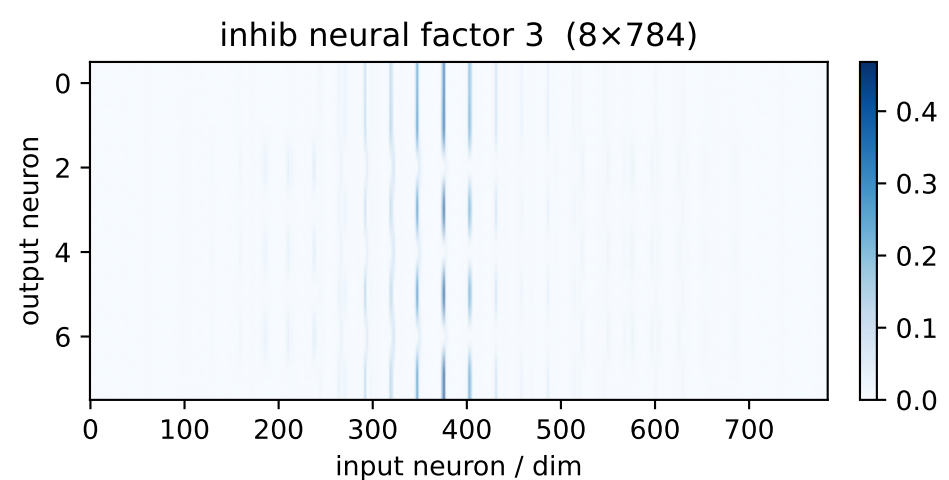
inh factor 3 \lambda=3.48 weighted avg
