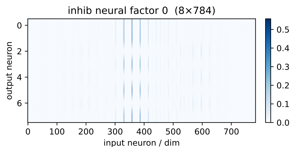
inh factor 0 \lambda=4.32 weighted avg
