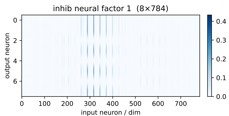
inh factor 1 \lambda=4.00 weighted avg
