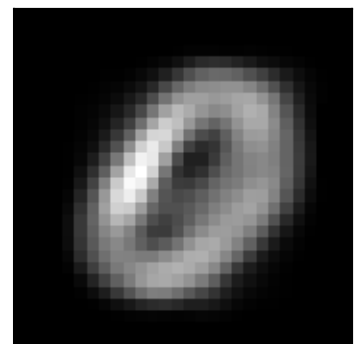
inh factor 3 \lambda=3.48 weighted avg
