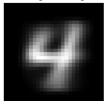
inh factor 2 \lambda=3.55 weighted avg
