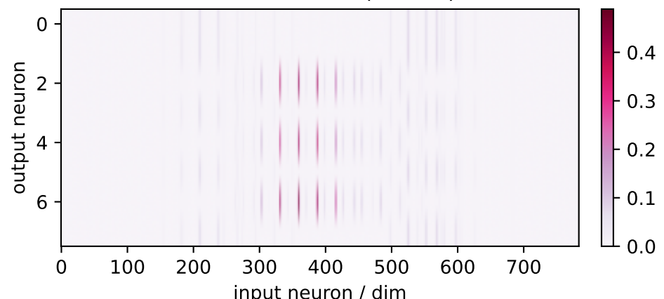
neural factor 3 (8×784)
