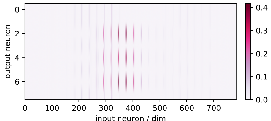
neural factor 1 (8×784)
