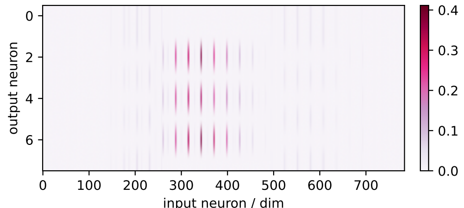
neural factor 2 (8×784)
