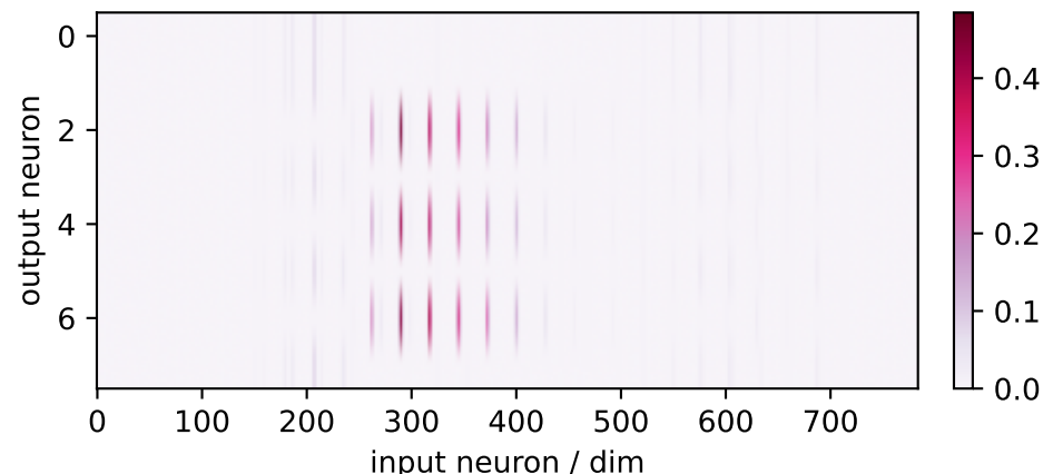
neural factor 0 (8×784)
