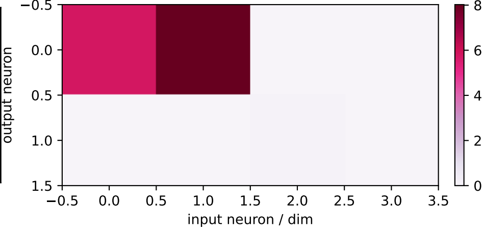
neural factor 1 (2×4)
