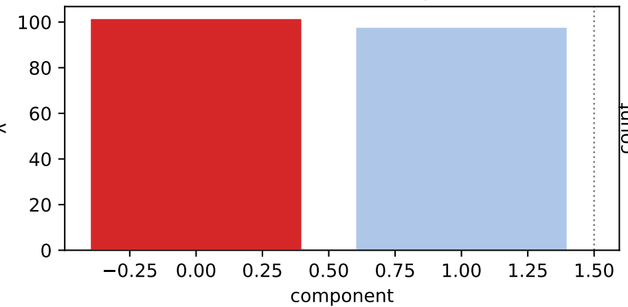
factor 0 \lambda=101.72 weighted avg
