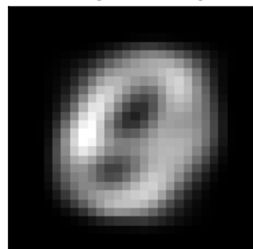
factor 1 \lambda=97.91 weighted avg
