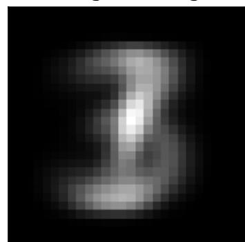
factor 0 \lambda=101.72 weighted avg
