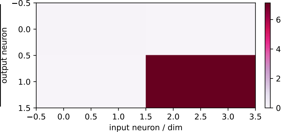
neural factor 0 (2×4)
