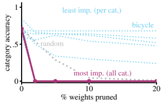
(c) causal pruning
