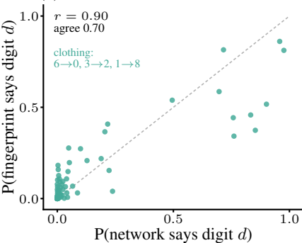
(g) mean fingerprint per condition
