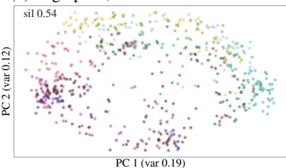
(g) ImageNet fingerprint, 253-d
