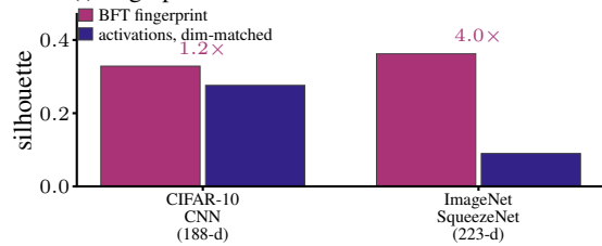
(i) fingerprint vs. activations
