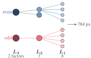
(a) 8x4 MLP trace: 13 factors
