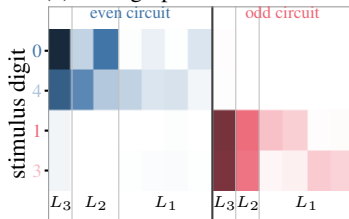
factor, by circuit and layer
