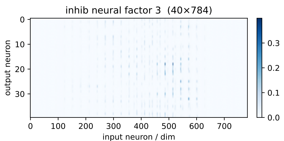
inh factor 3 \lambda=4.80 weighted avg
