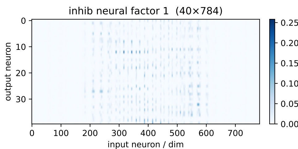
inh factor 1 \lambda=5.06 weighted avg
