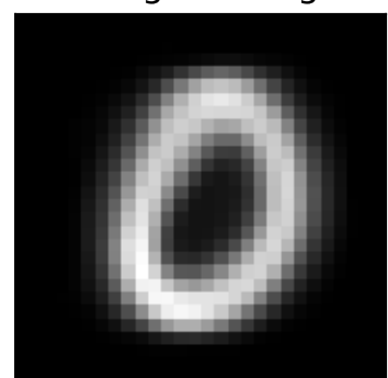
inh factor 3 \lambda=4.80 weighted avg
