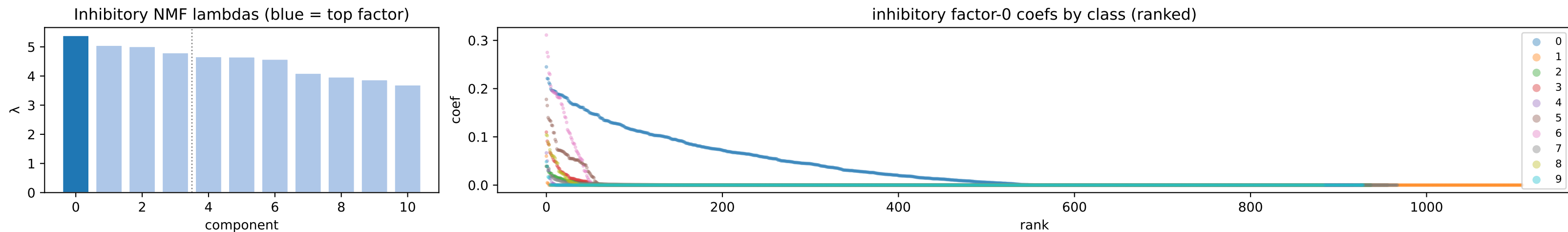
inh factor 0 \lambda=5.39 weighted avg
