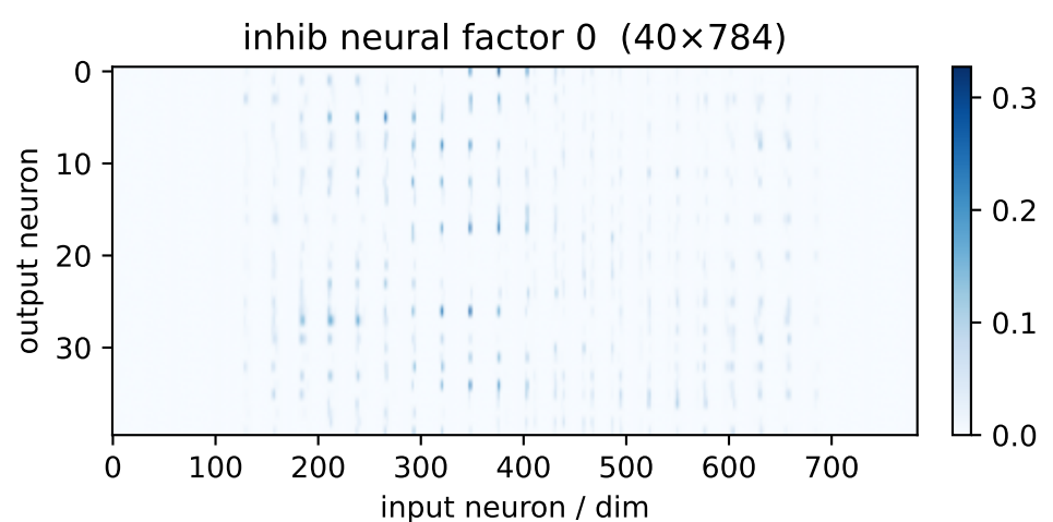
inh factor 0 \lambda=5.39 weighted avg
