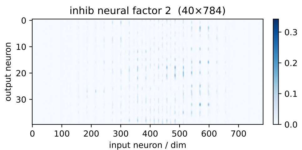
inh factor 2 \lambda=5.02 weighted avg
