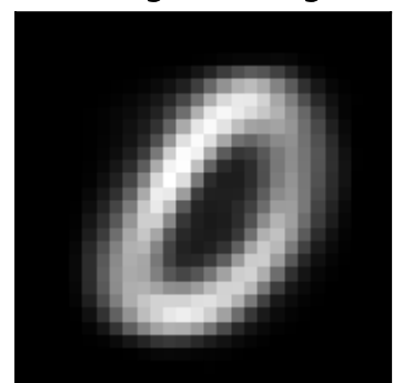
inh factor 0 \lambda=5.39 weighted avg
