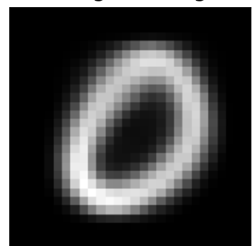
inh factor 2 \lambda=5.02 weighted avg
