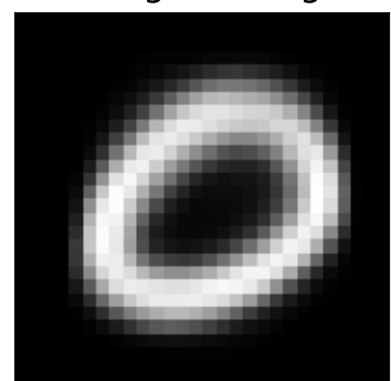
inh factor 1 \lambda=5.06 weighted avg
