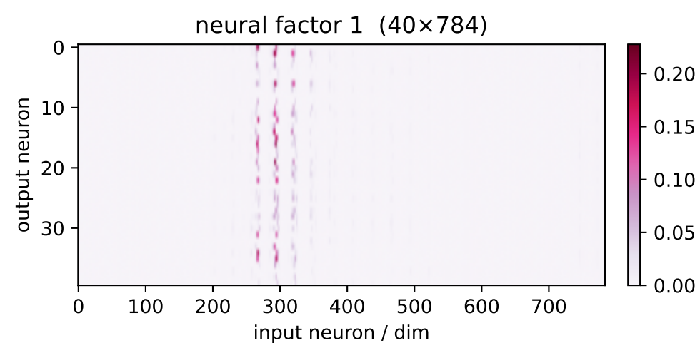
factor 1 \lambda=2.46 weighted avg
