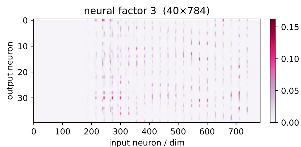
factor 3 \lambda=2.44 weighted avg
