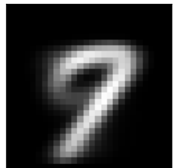
factor 3 \lambda=2.44 weighted avg
