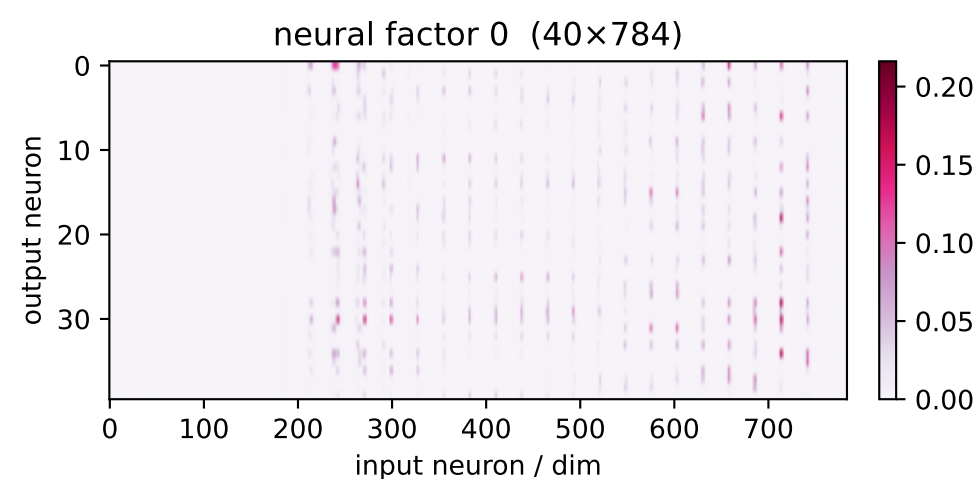
factor 0 \lambda=2.84 weighted avg
