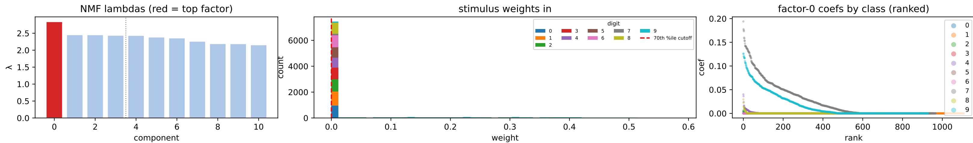
factor 0 \lambda=2.84 weighted avg
