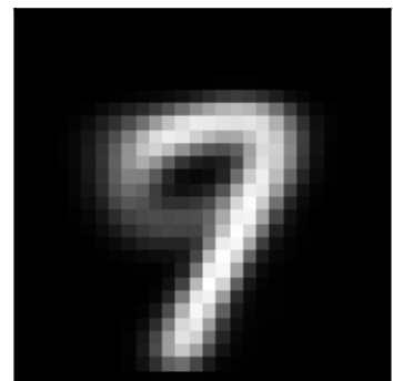
factor 0 \lambda=2.84 weighted avg
