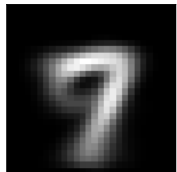
factor 1 \lambda=2.46 weighted avg
