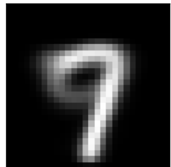
factor 2 \lambda=2.45 weighted avg
