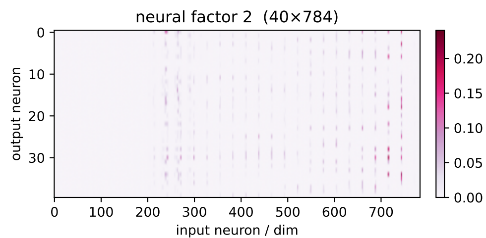
factor 2 \lambda=2.45 weighted avg
