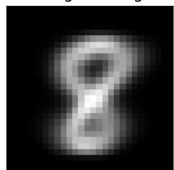
factor 3 \lambda=3.30 weighted avg
