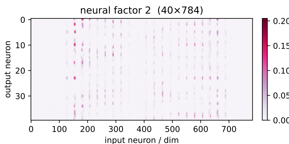
factor 2 \lambda=3.35 weighted avg
