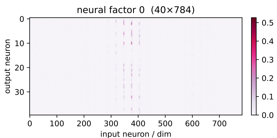
factor 0 \lambda=3.42 weighted avg
