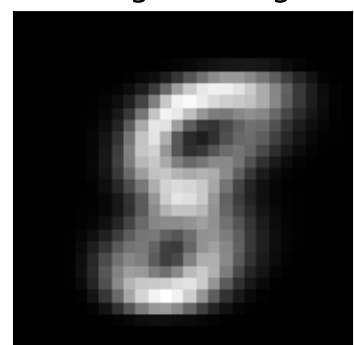
factor 1 \lambda=3.41 weighted avg
