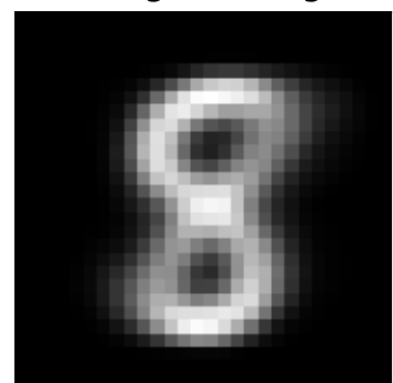
factor 2 \lambda=3.35 weighted avg
