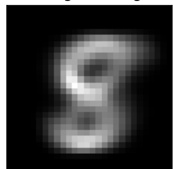
factor 0 \lambda=3.42 weighted avg
