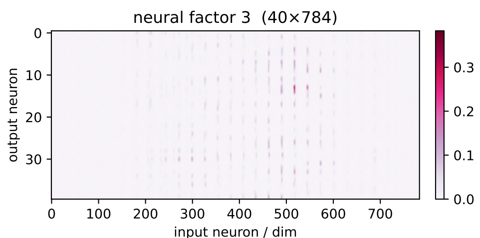
factor 3 \lambda=3.30 weighted avg
