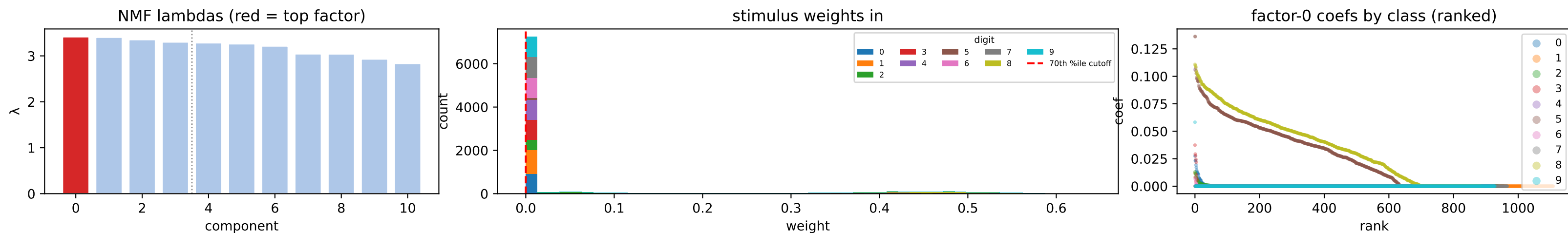
factor 0 \lambda=3.42 weighted avg
