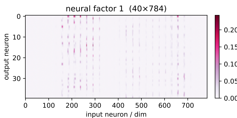
factor 1 \lambda=3.41 weighted avg
