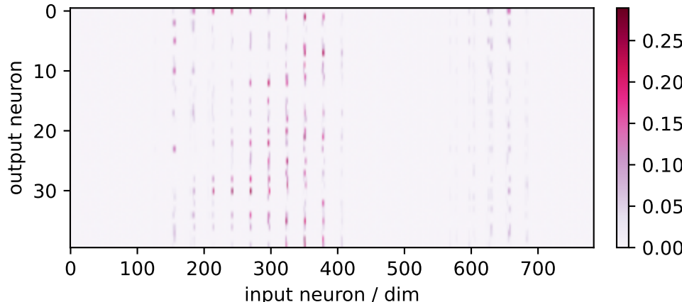
neural factor 0 (40×784)
