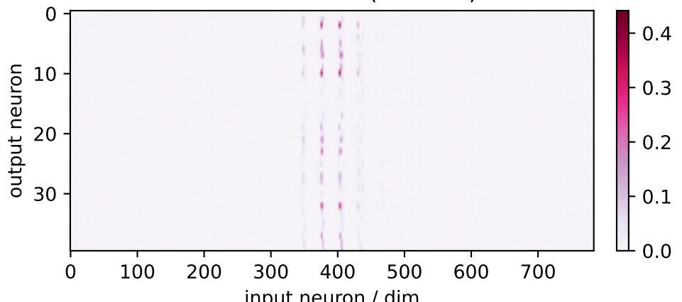
neural factor 3 (40×784)
