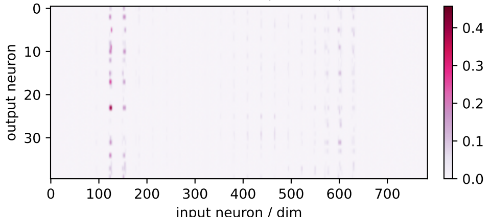
neural factor 1 (40×784)
