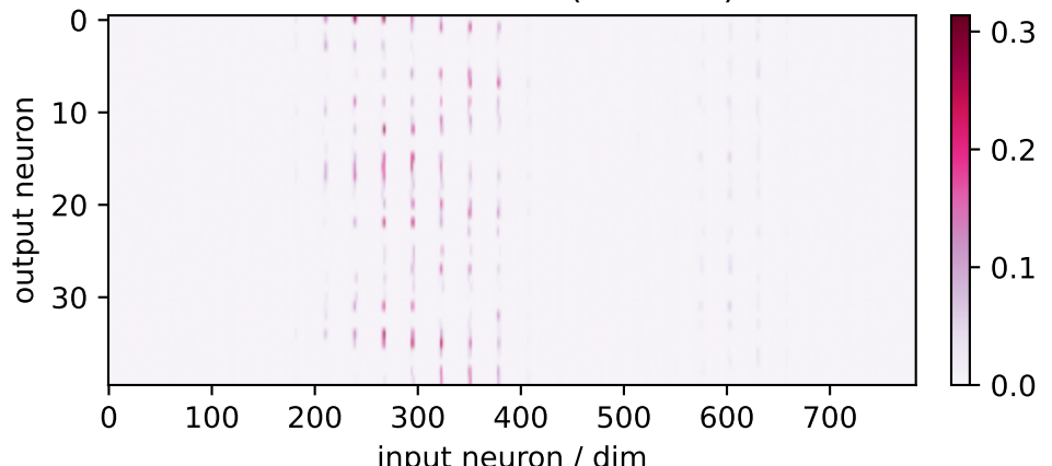
neural factor 2 (40×784)
