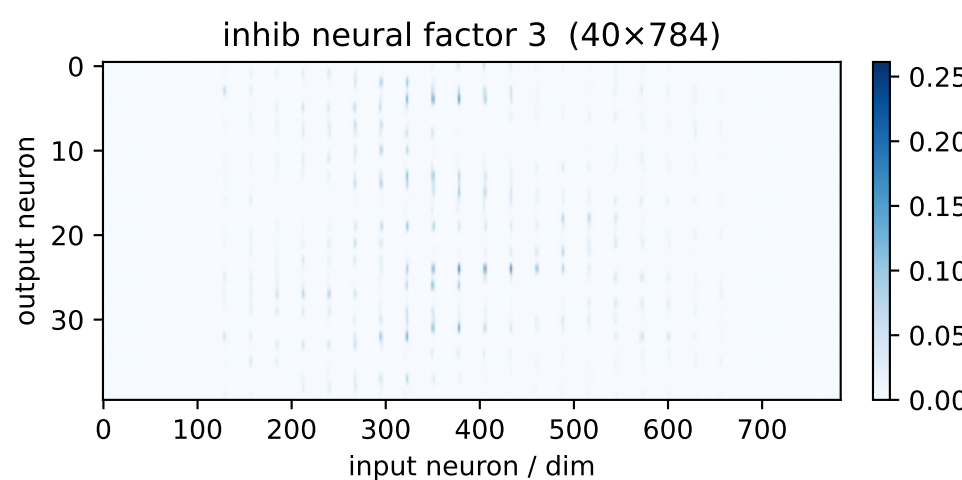
inh factor 3 \lambda=1.99 weighted avg
