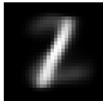
inh factor 3 \lambda=1.99 weighted avg
