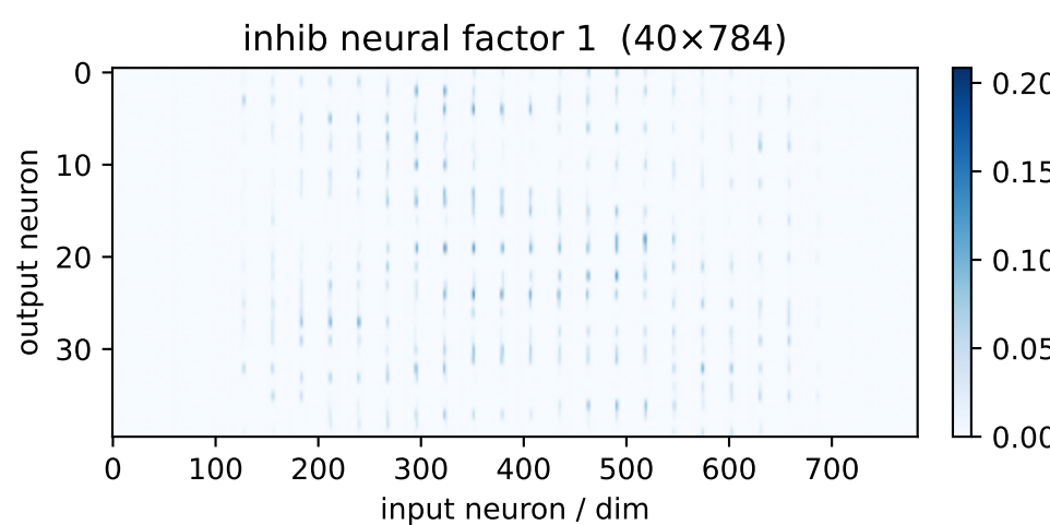
inh factor 1 \lambda=2.72 weighted avg
