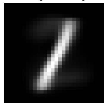
inh factor 0 \lambda=3.09 weighted avg
