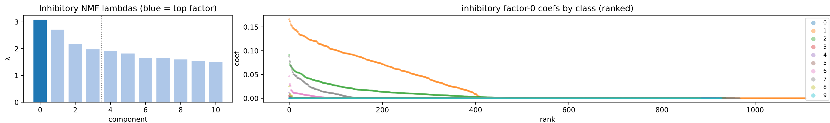
inh factor 0 \lambda=3.09 weighted avg
