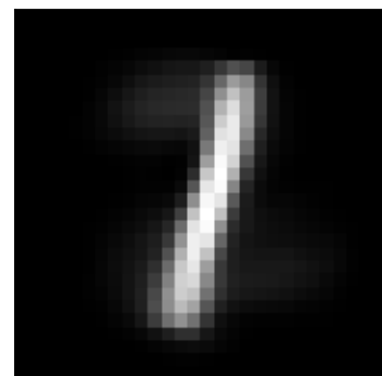
inh factor 1 \lambda=2.72 weighted avg
