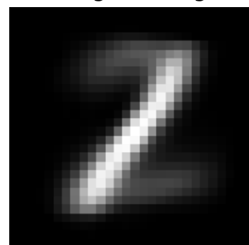
inh factor 2 \lambda=2.19 weighted avg
