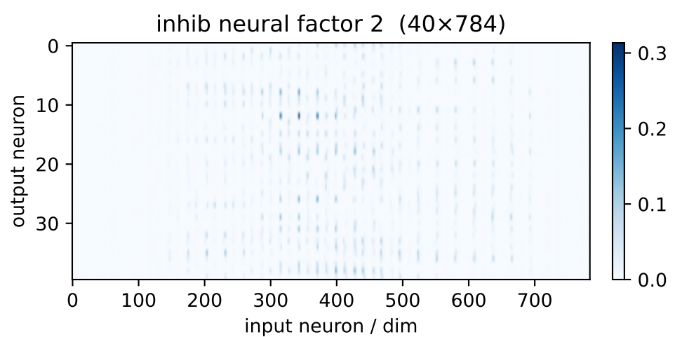
inh factor 2 \lambda=4.36 weighted avg
