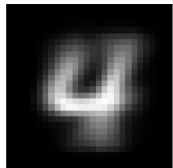
inh factor 1 \lambda=4.81 weighted avg
