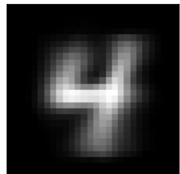
inh factor 3 \lambda=4.23 weighted avg
