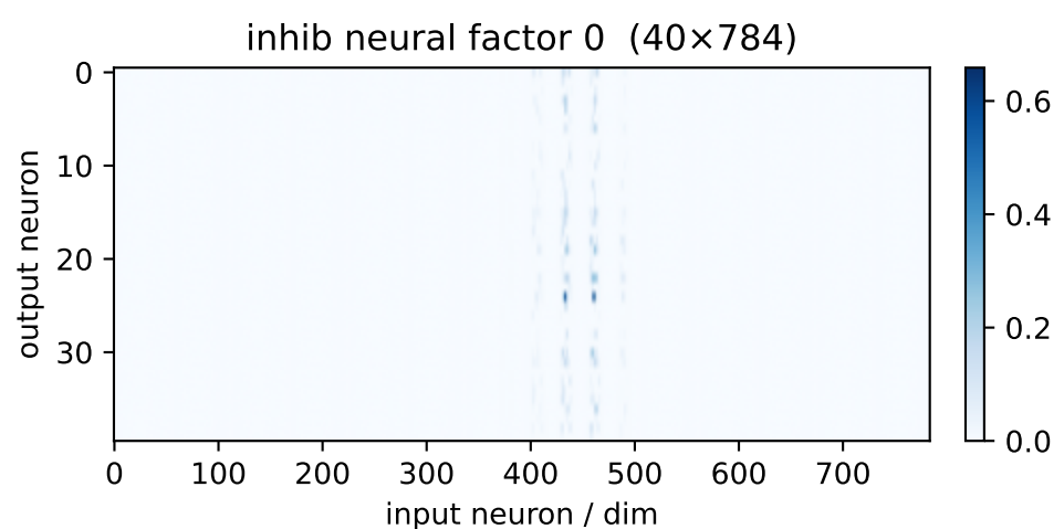
inh factor 0 \lambda=5.07 weighted avg
