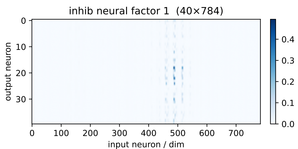
inh factor 1 \lambda=4.81 weighted avg
