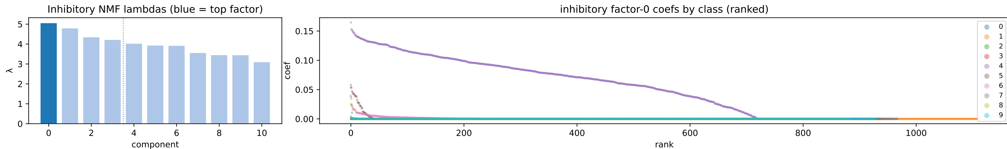
inh factor 0 \lambda=5.07 weighted avg
