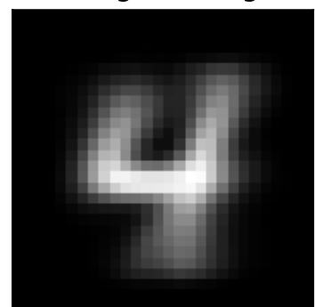
inh factor 0 \lambda=5.07 weighted avg
