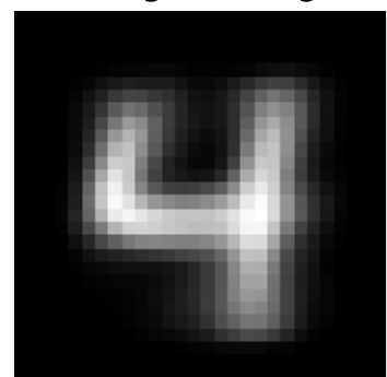
inh factor 2 \lambda=4.36 weighted avg
