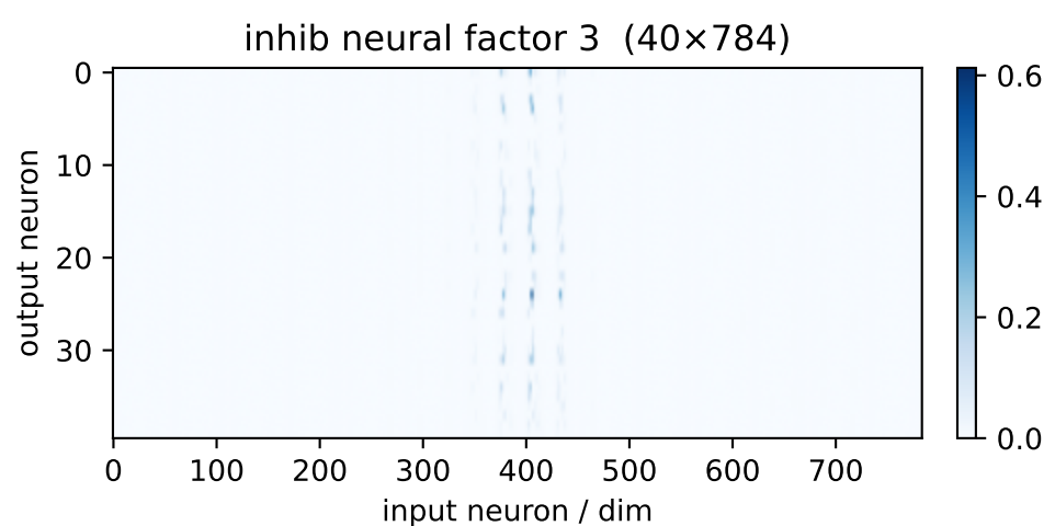
inh factor 3 \lambda=4.23 weighted avg
