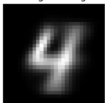
factor 2 \lambda=4.21 weighted avg
