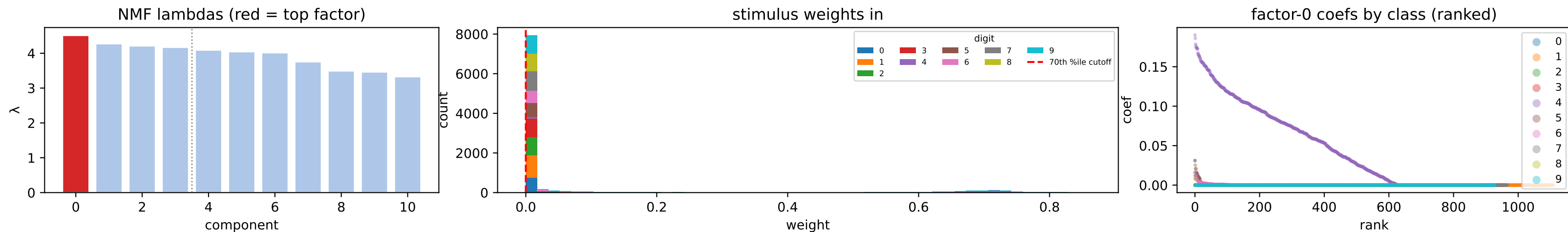
factor 0 \lambda=4.51 weighted avg
