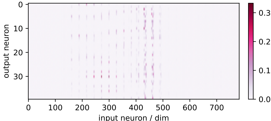
neural factor 0 (40×784)
