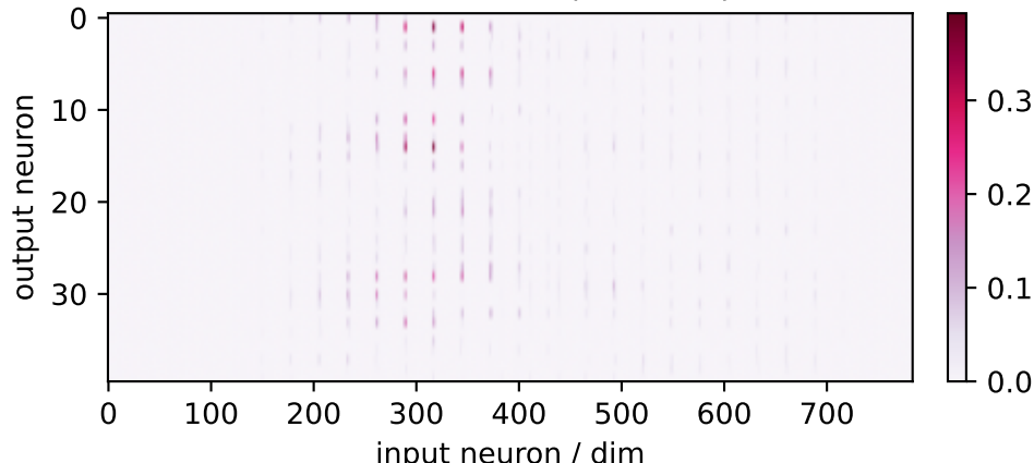
neural factor 1 (40×784)
