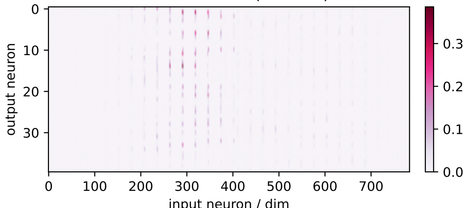
neural factor 2 (40×784)
