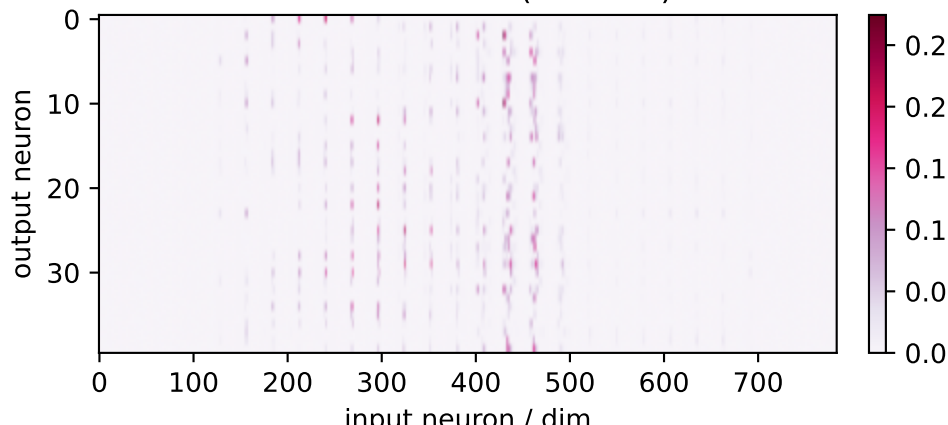
neural factor 3 (40×784)
