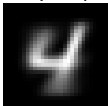
factor 0 \lambda=4.51 weighted avg
