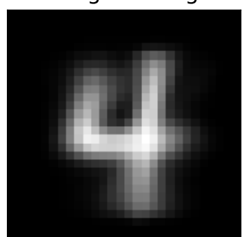
factor 3 \lambda=4.17 weighted avg
