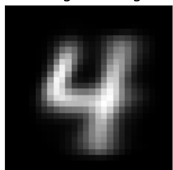
factor 1 \lambda=4.27 weighted avg
