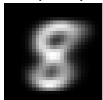
inh factor 0 \lambda=11.26 weighted avg
