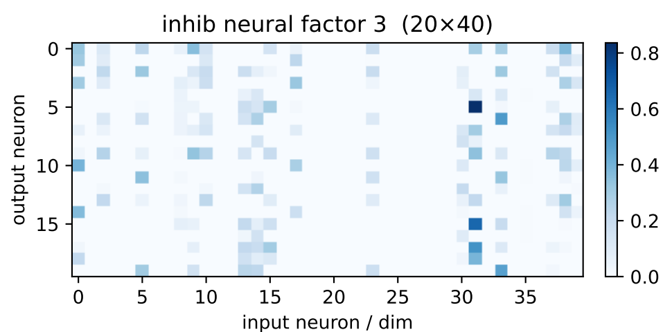
inh factor 3 \lambda=6.94 weighted avg
