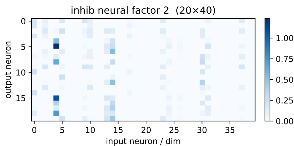
inh factor 2 \lambda=7.24 weighted avg
