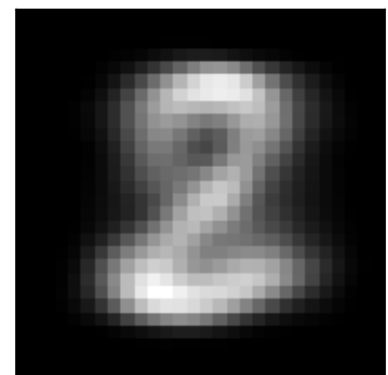
inh factor 3 \lambda=6.94 weighted avg
