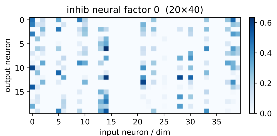
inh factor 0 \lambda=11.26 weighted avg
