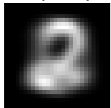
inh factor 2 \lambda=7.24 weighted avg
