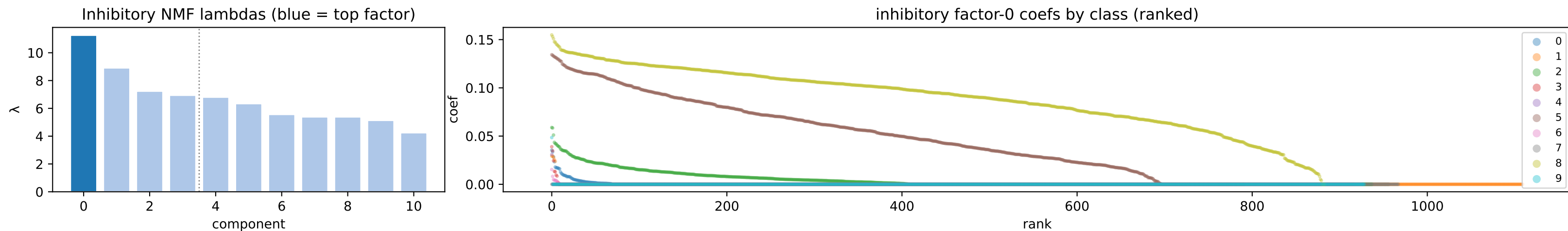
inh factor 0 \lambda=11.26 weighted avg
