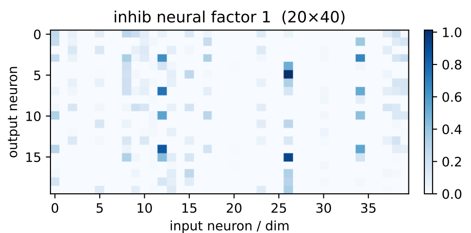
inh factor 1 \lambda=8.91 weighted avg
