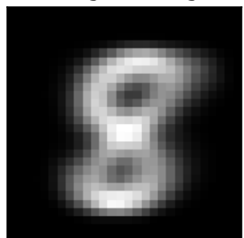
factor 0 \lambda=13.10 weighted avg
