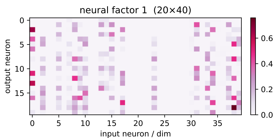
factor 1 \lambda=8.80 weighted avg
