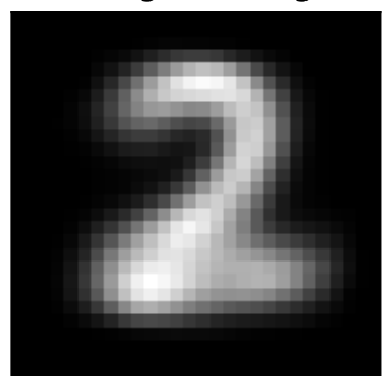
factor 2 \lambda=7.91 weighted avg
