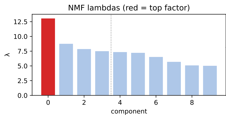
factor 0 \lambda=13.10 weighted avg
