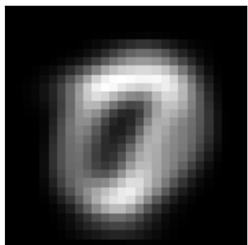
factor 1 \lambda=164.91 weighted avg
