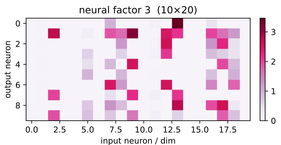
factor 3 \lambda=156.14 weighted avg
