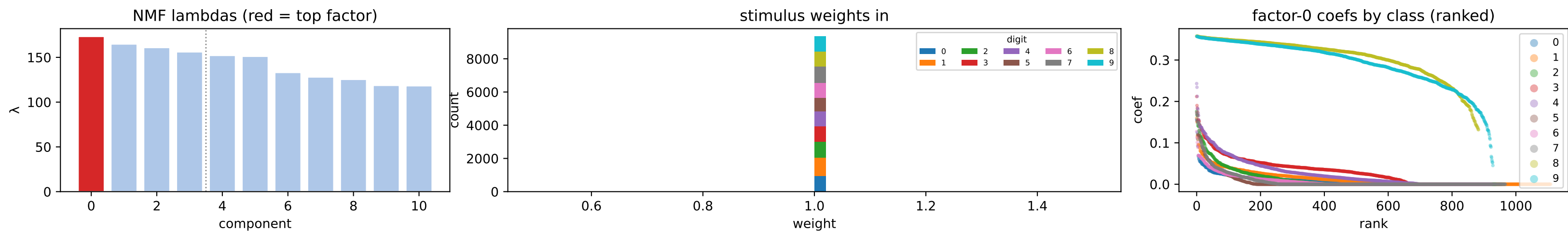
factor 0 \lambda=173.40 weighted avg
