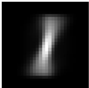
factor 3 \lambda=156.14 weighted avg
