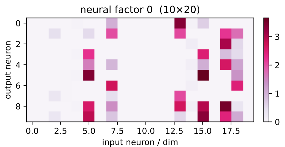
factor 0 \lambda=173.40 weighted avg
