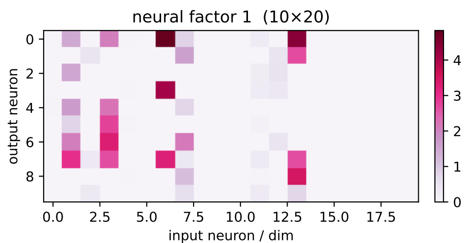
factor 1 \lambda=164.91 weighted avg
