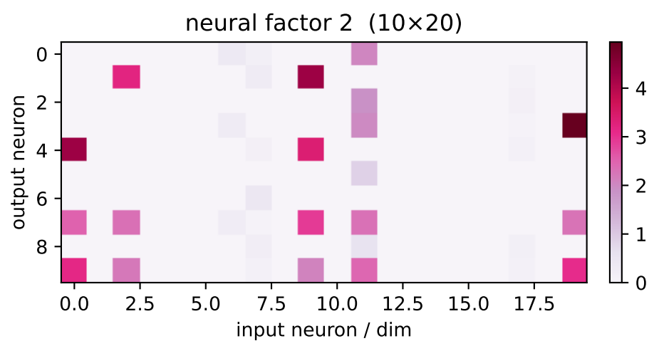
factor 2 \lambda=160.97 weighted avg
