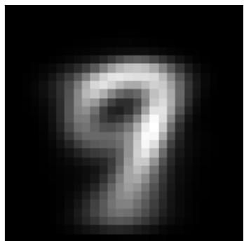
factor 2 \lambda=160.97 weighted avg
