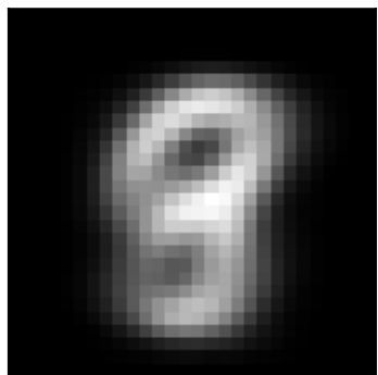
factor 0 \lambda=173.40 weighted avg
