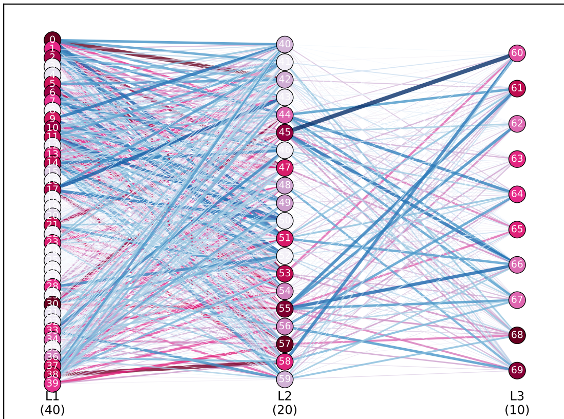
Factor Trace — Network Scaffold [path: F0→F0] (NMF factor at each layer, traced backwards from output)
