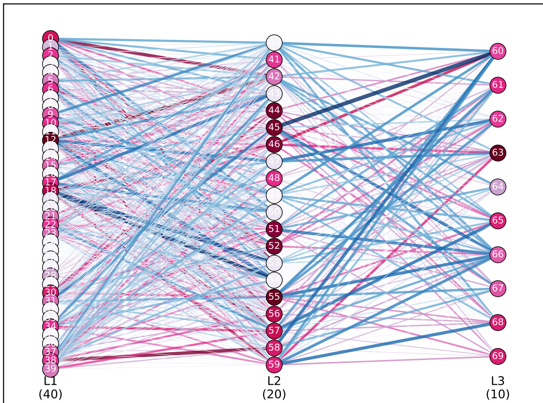
Factor Trace — Network Scaffold [path: F6→F0] (NMF factor at each layer, traced backwards from output)
