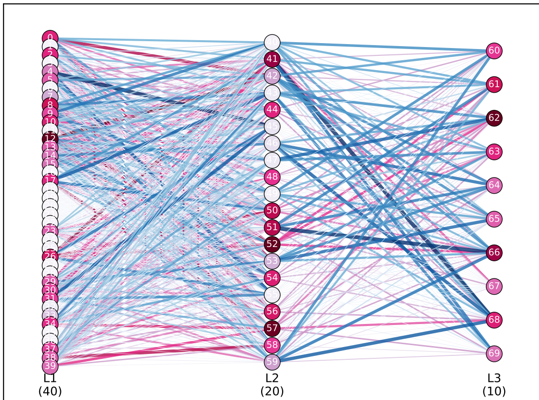
Factor Trace — Network Scaffold [path: F7→F0] (NMF factor at each layer, traced backwards from output)
