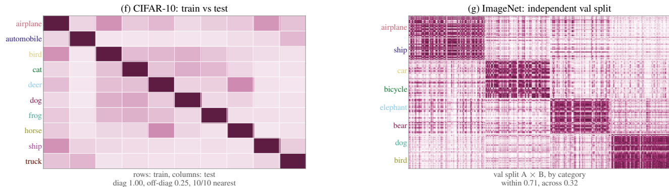
(f,g) the code is a property of the class, not the sample
