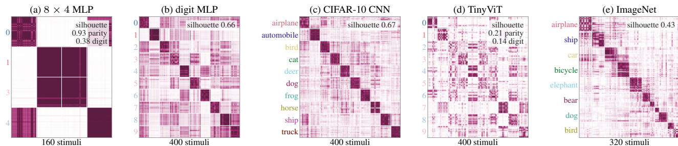
(a–e) class geometry: pairwise cosine of the fingerprints, sorted by class
