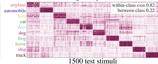
(i) both · fingerprint vs. activations
