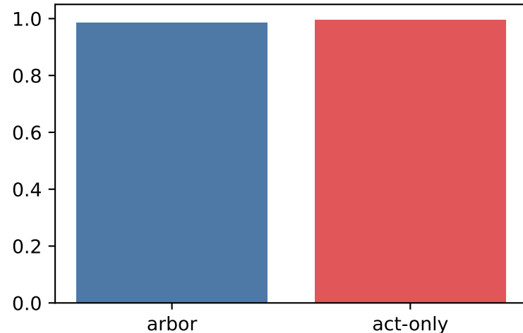
fingerprint kNN
