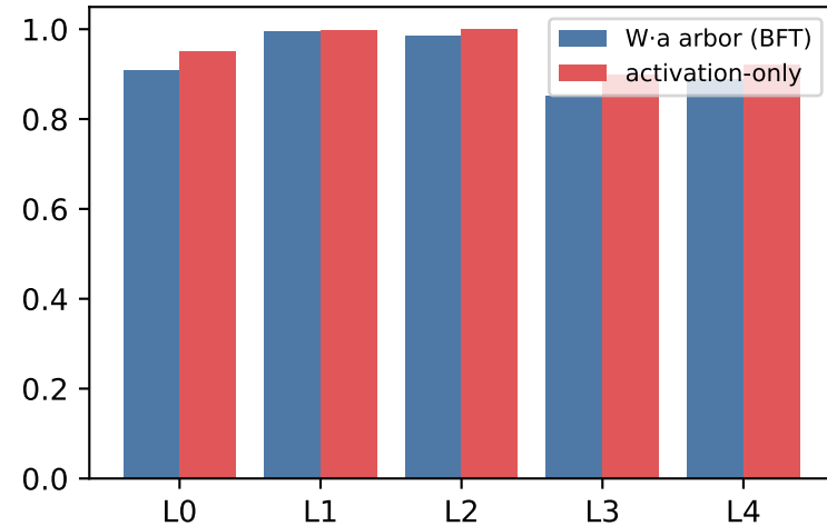
NMF stability
