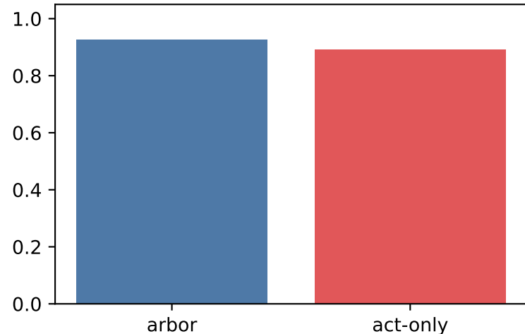
fingerprint kNN
