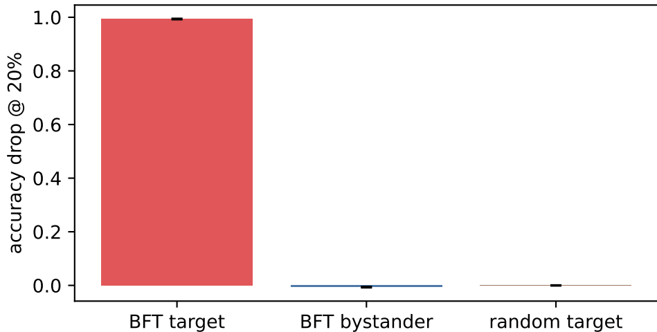
Circuit ablation — mlp_even_odd (library weight-level (bft_top); Wilcoxon p=0.5 )
