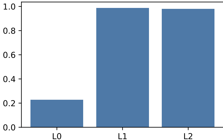
pre-activation R^2
