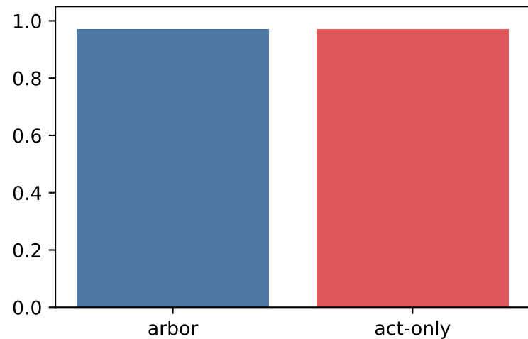
fingerprint kNN
