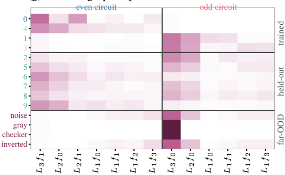
(g) mean fingerprint per condition
