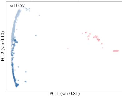
(a) fingerprint embedding
