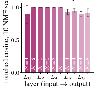
(g) vs. baselines: fingerprint or activations
