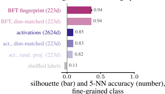
(g) vs. baselines: fingerprint or activations
