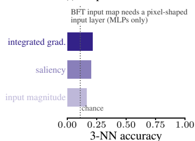
(i) vs. pixel attribution
