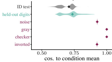
(f) far-OOD collapse
