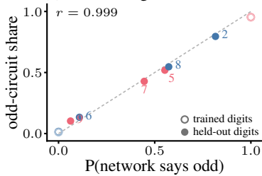
(e) held-out digits
